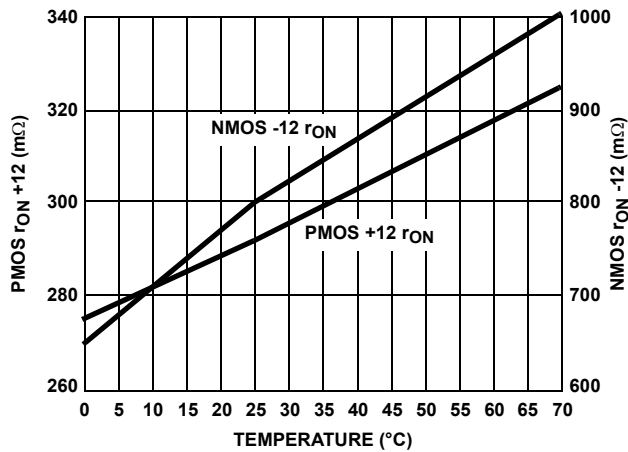
FIGURE 4. r_{ON} vs TEMPERATURE
