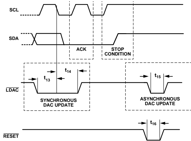
Figure 5. \bar{P}C , LDAC, and RESET Timing
