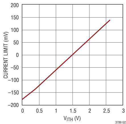
Peak Current Threshold vs V_{\text{ITH}} (Boost)
