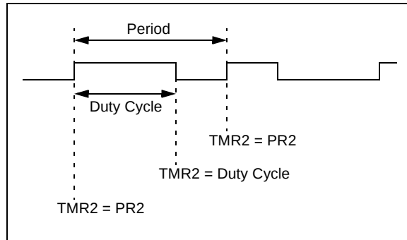
FIGURE 8-4: PWM OUTPUT
