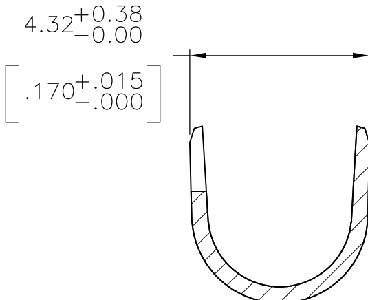
SECTION X-X
