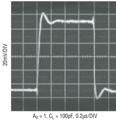
Small-Signal Response
