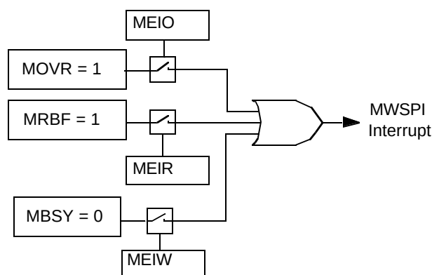
Figure 30. MWSPi Interrupts
