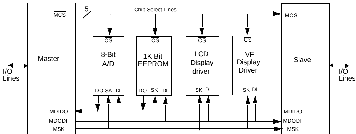
Figure 24. MICROWIRE Interface
