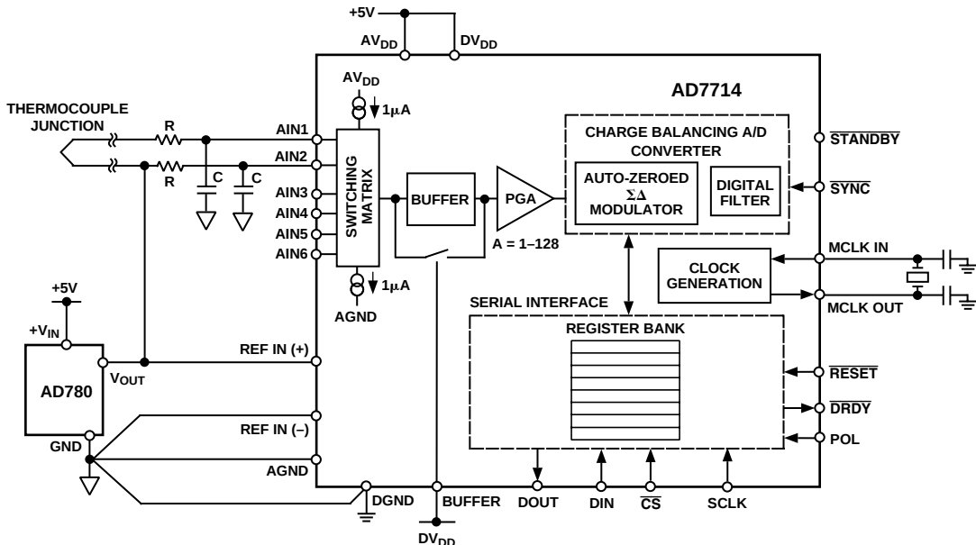
Figure 13. Thermocouple Measurement Using the AD7714
