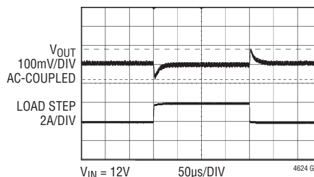
12V Input to 1.8V Output, 50% Load Transient Response
