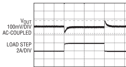
12V Input to 1.8V Output, 50% Load Transient Response
