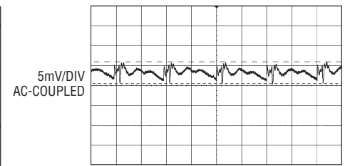
Output Ripple
