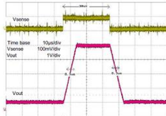
Figure 12: Step response
