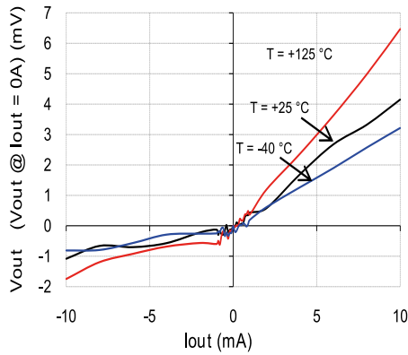
Figure 11: Output stage load regulation
