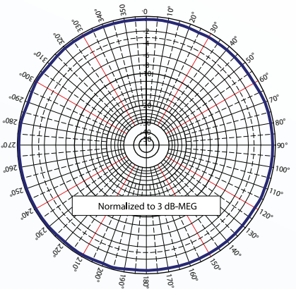
Azimuth Pattern (X,Y, or E-plane)
