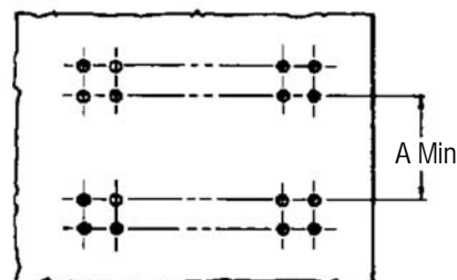
Side-to-Side Clearance
