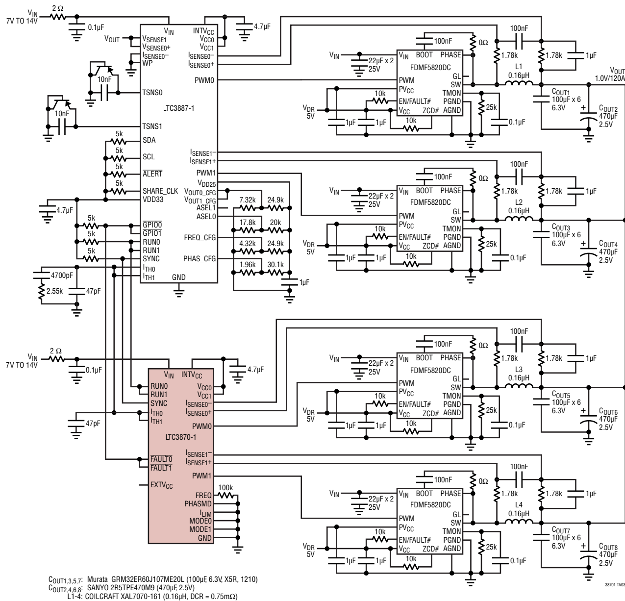
High Efficiency 425kHz 4-Phase 1.0V Step-Down Converter
