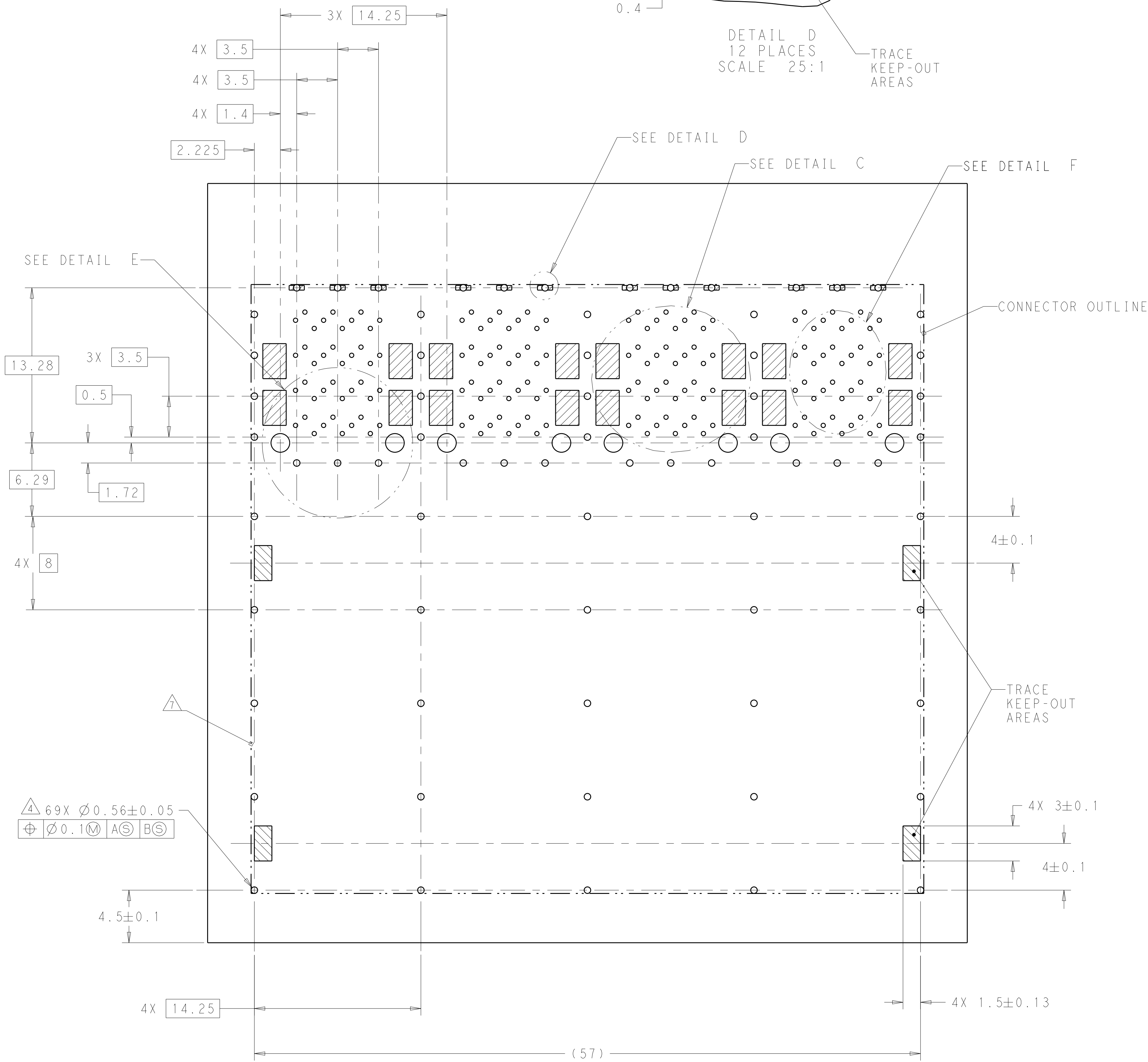
RECOMMENDED PCB LAYOUT SCALE 5:1
