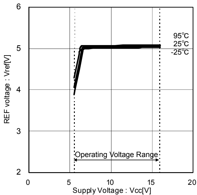
Fig.4 Reference voltage
