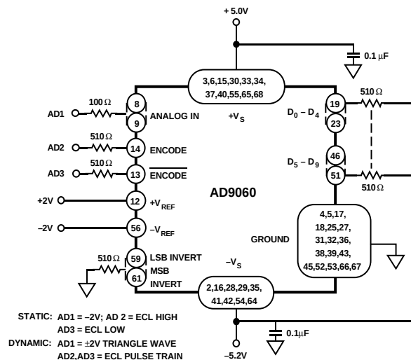
AD9060 Burn-In Connections
