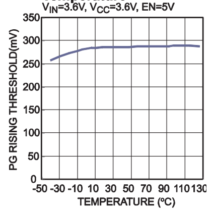
PG Rising Threshold vs. Temperature
