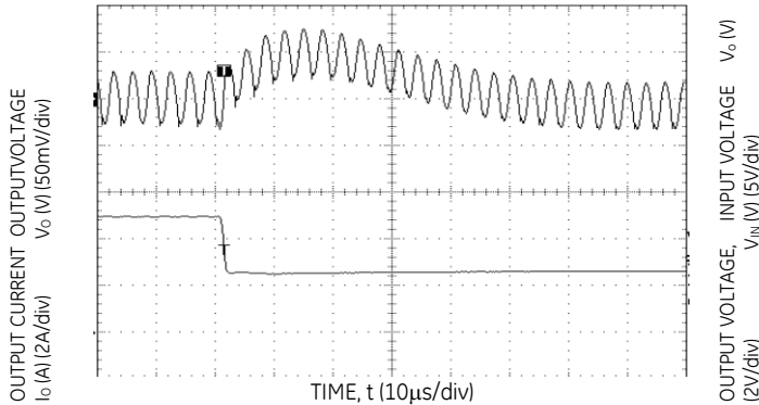
Figure 13. Transient Response to Dynamic Load Change from 100% of 50% full load ( V_o = 5.0 Vdc, C_{ext} = 2 \times 150 µF Polymer Capacitors).
