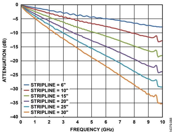
Figure 148. Insertion Loss of 50 \Omega Striplines on FR4
