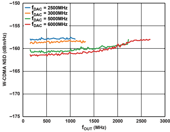
Figure 24. W-CDMA NSD Measured at 70 MHz vs. f_{OUT} over f_{DAC}
