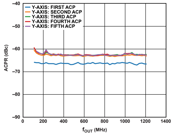
Figure 55. 32-Carrier ACPR vs. f_{OUT}
