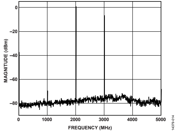
Figure 67. Single-Tone Spectrum at f_{OUT} = 2000 \text{ MHz}
