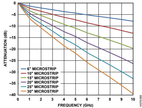
Figure 149. Insertion Loss of 50 Ohm Microstrips on FR4
