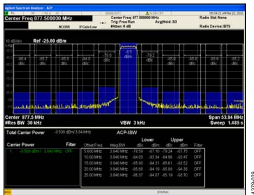
Figure 84. Single-Carrier W-CDMA at 877.5 MHz
