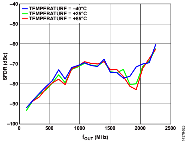
Figure 76. SFDR vs. f_{OUT} over Temperature
