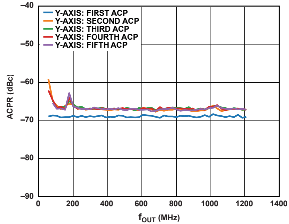
Figure 54. 16-Carrier ACPR vs. f_{OUT}
