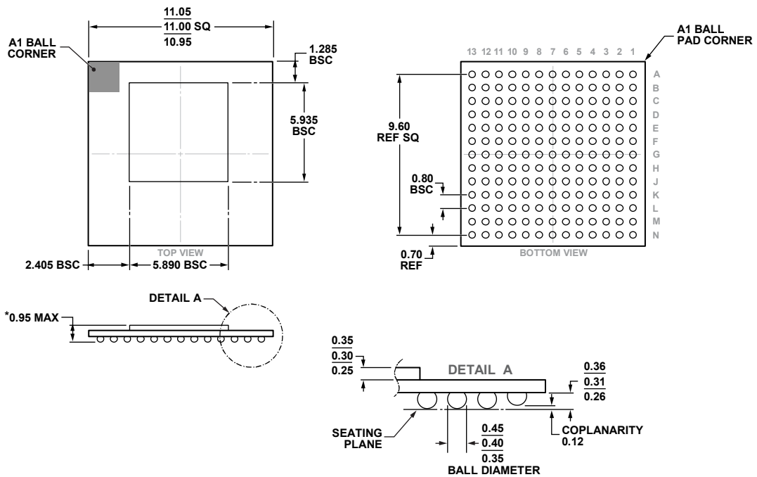
Figure 195. 165-Ball Chip Scale Package Ball Grid Array [CSP_BGA] (BC-165-1) Dimensions shown in millimeters
