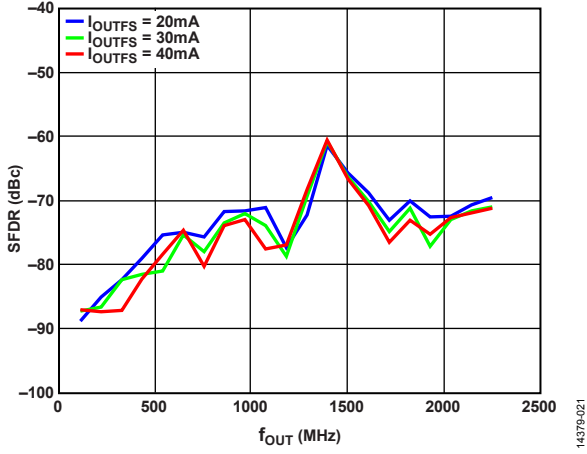
Figure 74. SFDR vs. f_{OUT} over DAC I_{OUTFS}
