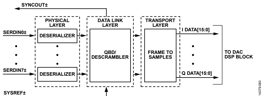
Figure 143. Functional Block Diagram of Serial Link Receiver
