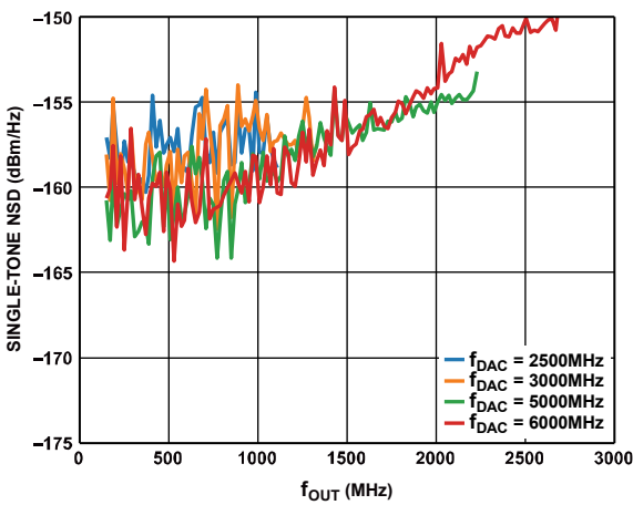
Figure 20. Single-Tone NSD Measured at 70 MHz vs. f_{OUT} over f_{DAC}
