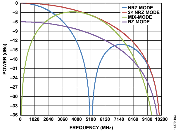
Figure 184. Sinc Roll-Off with 2 \times NRZ Mode Added, f_{DAC} = 5.1 GSPS
