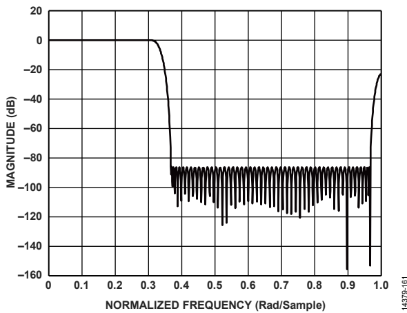
Figure 167. 3x Third-Band 90% Filter Response
