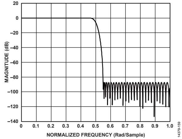
Figure 165. First 2x Half-Band 90% Filter Response
