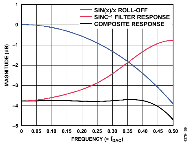
Figure 173. Responses of \text{Sin}(x)/x Roll-Off, the \text{Sinc}^{-1} Filter, and the Composite of the Two
