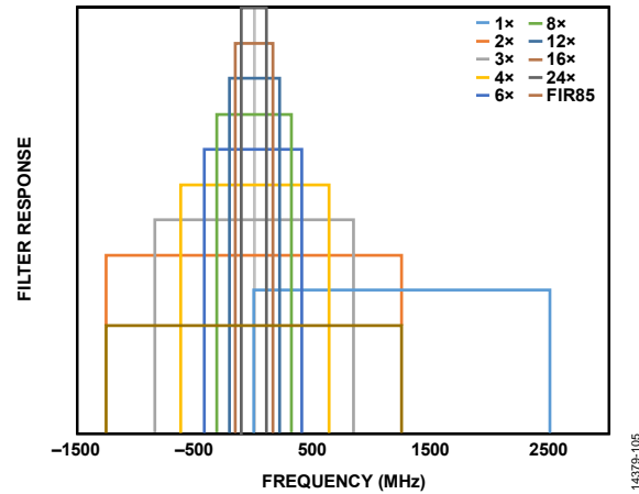
Figure 162. All Band Responses of Interpolation Filters
