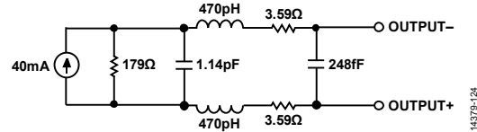
Figure 193. Equivalent Circuit Model of the DAC Output
