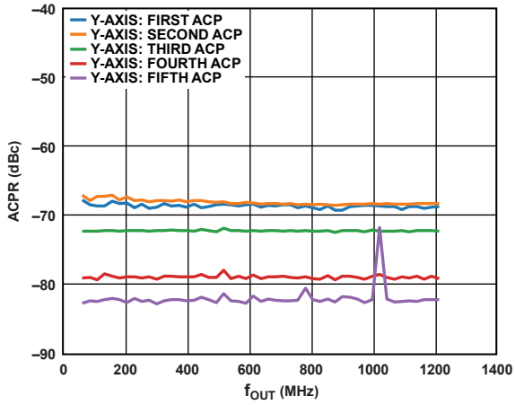
Figure 51. Single-Carrier Adjacent Channel Power Ratio (ACPR) vs. f_{OUT}
