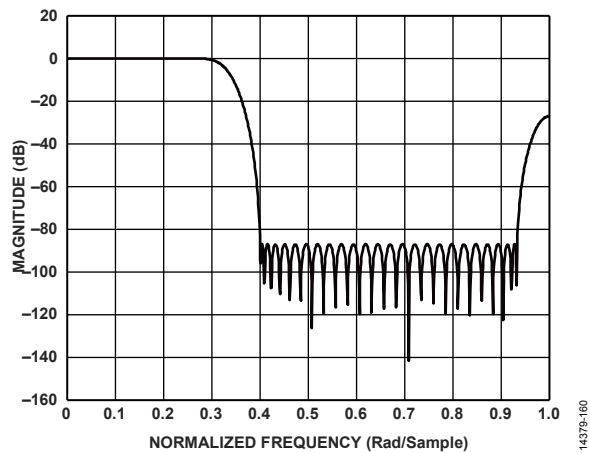
Figure 166. 3x Third-Band 80% Filter Response
