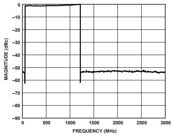
Figure 56. 194-Carrier, Sinc On, FIR85 Enabled
