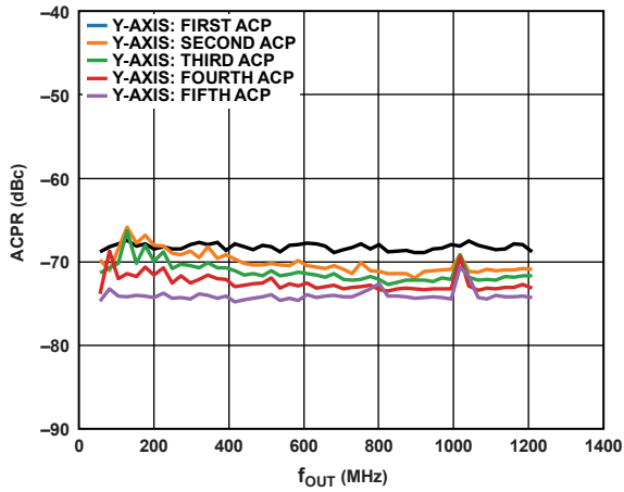
Figure 52. Four-Carrier ACPR vs. f_{OUT}
