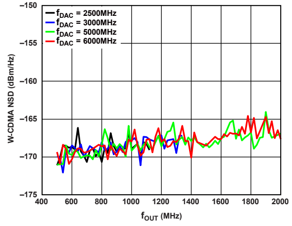
Figure 80. W-CDMA NSD Measured at 10% Offset from f_{OUT} vs. f_{OUT} over f_{DAC}
