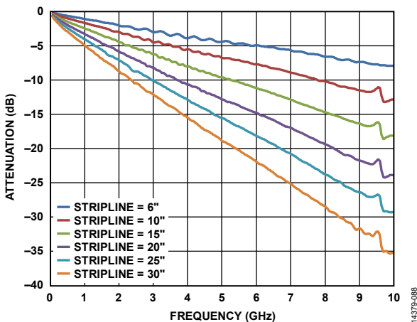
Figure 148. Insertion Loss of 50 Ohm Striplines on FR4
