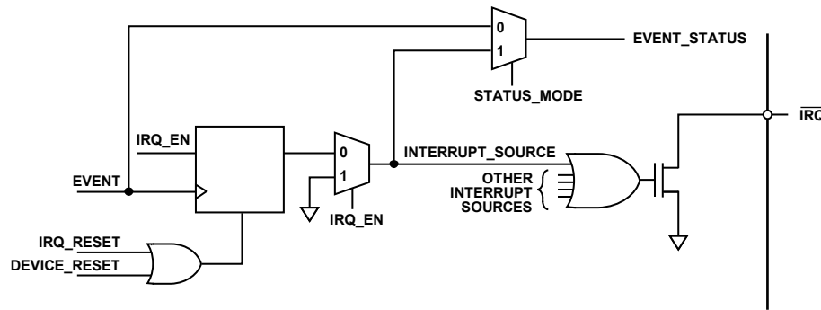
Figure 175. Simplified Schematic of \overline{\text{IRQ}} Circuitry
