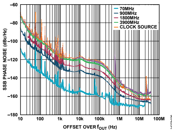
Figure 93. SSB Phase Noise vs. Offset over f_{OUT} , f_{DAC} = 6000 \text{ MSPS}
