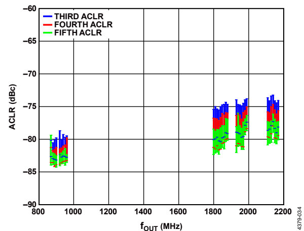
Figure 92. Two-Carrier, W-CDMA ACLR vs. f_{OUT} (Third ACLR, Fourth ACLR, Fifth ACLR)
