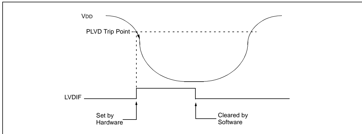
FIGURE 8-2: PLVD OPERATION
