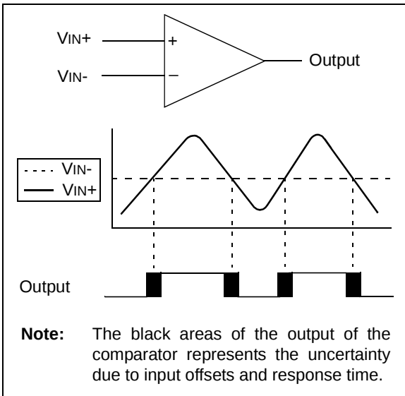
FIGURE 7-1: SINGLE COMPARATOR
