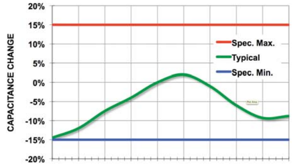
MAXICAP TEMPERATURE COEFFICIENT
