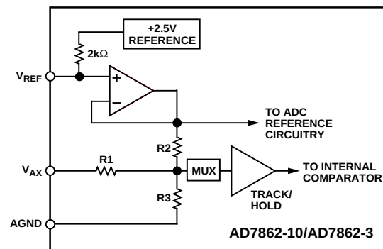
Figure 3 shows the analog input section for the AD7862-10 and AD7862-3. The analog input range of the AD7862-10 is \pm 10 V into an input resistance of typically 33 k \Omega . The analog input range of the AD7862-3 is \pm 2.5 V into an input resistance of typically 12 k \Omega . This input is benign with no dynamic charging
