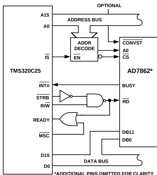
Figure 16. AD7862-TMS320C25 Interface
