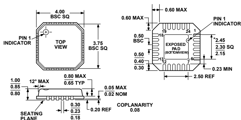
Figure 43. 24-Lead Lead Frame Chip Scale Package [LFCSP_VQ] 4 mm x 4 mm Body, Very Thin Quad (CP-24-2) Dimensions shown in millimeters
