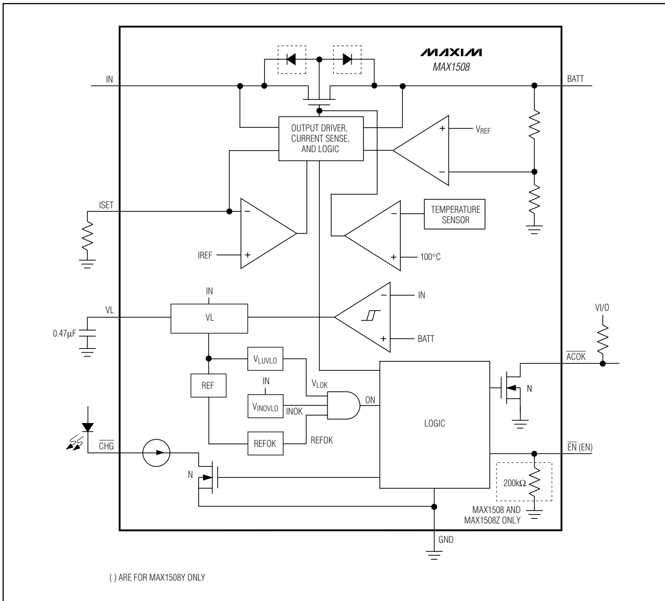
Figure 1. Functional Diagram
