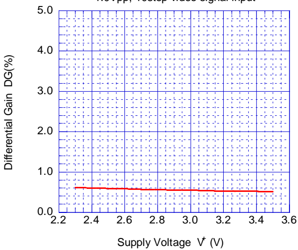
Differential Gain vs. Supply Voltage 1.0Vpp, 10step video signal input
