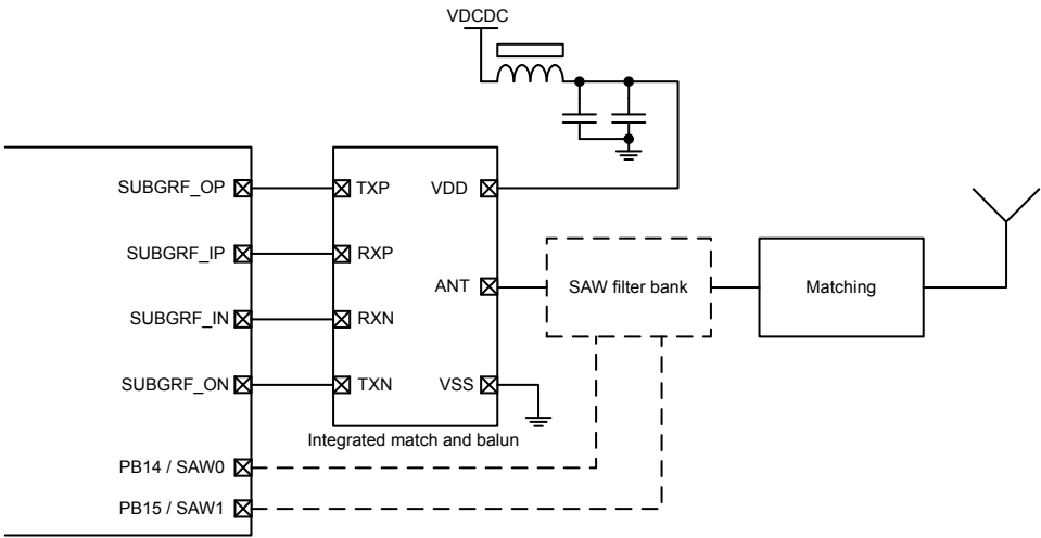
Figure 3.2. Radio Interface
