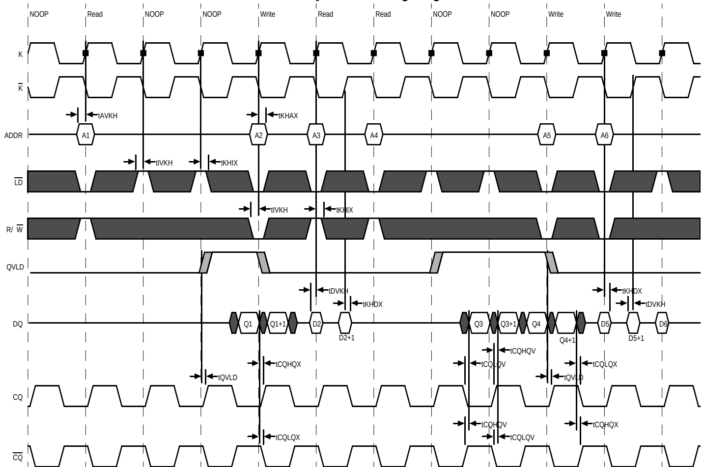
Read-Write CQ-Based Timing Diagram
