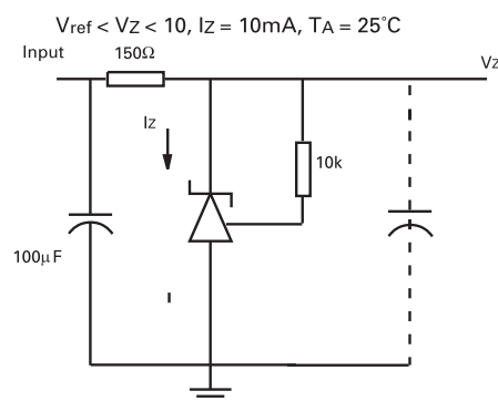
Test Circuit for Stability Boundary Conditions
