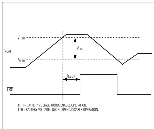
Figure 8. Hysteresis
