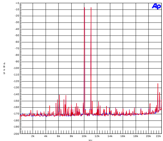
Figure 53. IMD – 10 kHz and 11 kHz -7 dBFS, 48 kHz:44.1 kHz
