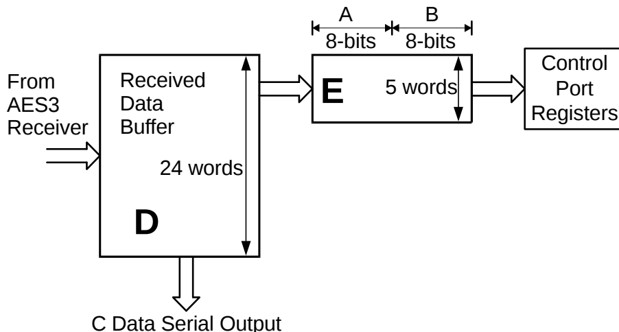
Figure 34. Channel Status Data Buffer Structure
