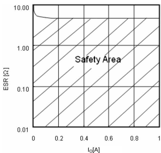
Fig.19 ESR condencer
