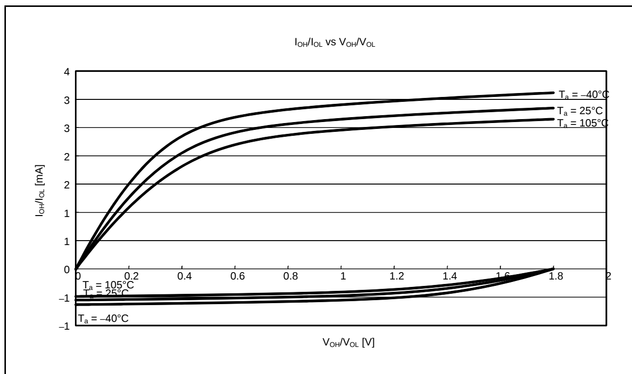
Figure 5.15 V_{OH}/V_{OL} and I_{OH}/I_{OL} Temperature Characteristics of Port 4 and Port J at V_{CC} = 1.8\text{ V} (Reference Data)
