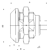
ER : Fixed receptacle, front panel mounting
