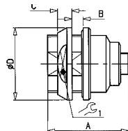
EP : Fixed receptacle, back panel mounting
