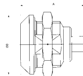
ER : Fixed receptacle, front panel mounting
