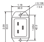
SUGGESTED MOUNTING CUTOUT (MOUNTING FROM BEHIND)
