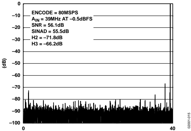
Figure 15. FFT: FS = 80 MSPS, A_{IN} = 39 MHz @ -0.5 dBFS, Differential, 1 V p-p Input Range
