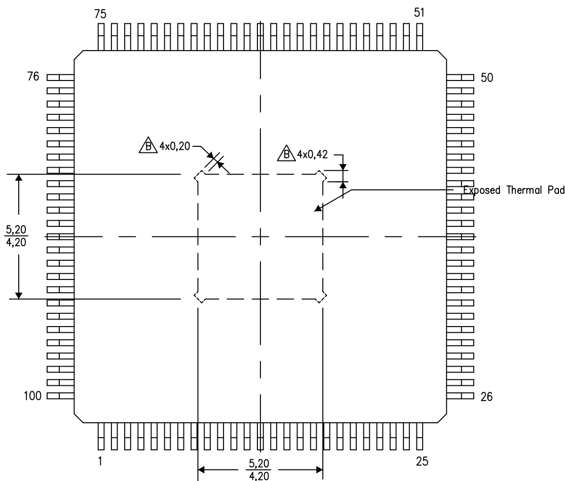
Top View
