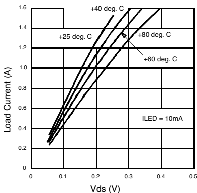
Figure 3. Typical On-Characteristics
