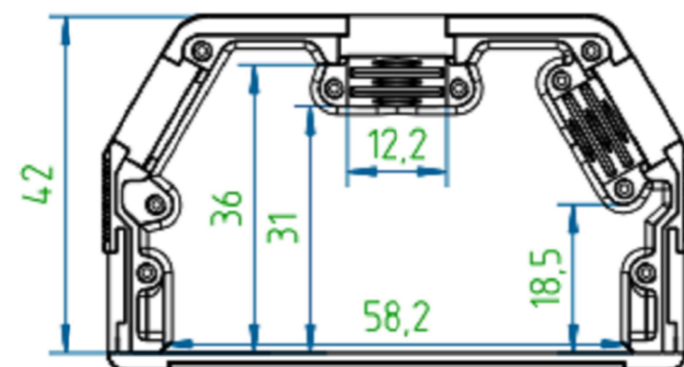
CABLE BUSHING
