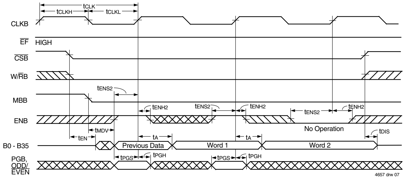
Figure 4. FIFO Read Cycle Timing
