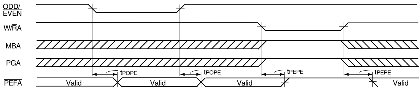
Figure 11. ODD/ \overline{EVEN} , W/RA, MBA, and PGA to \overline{PEFA} Timing
