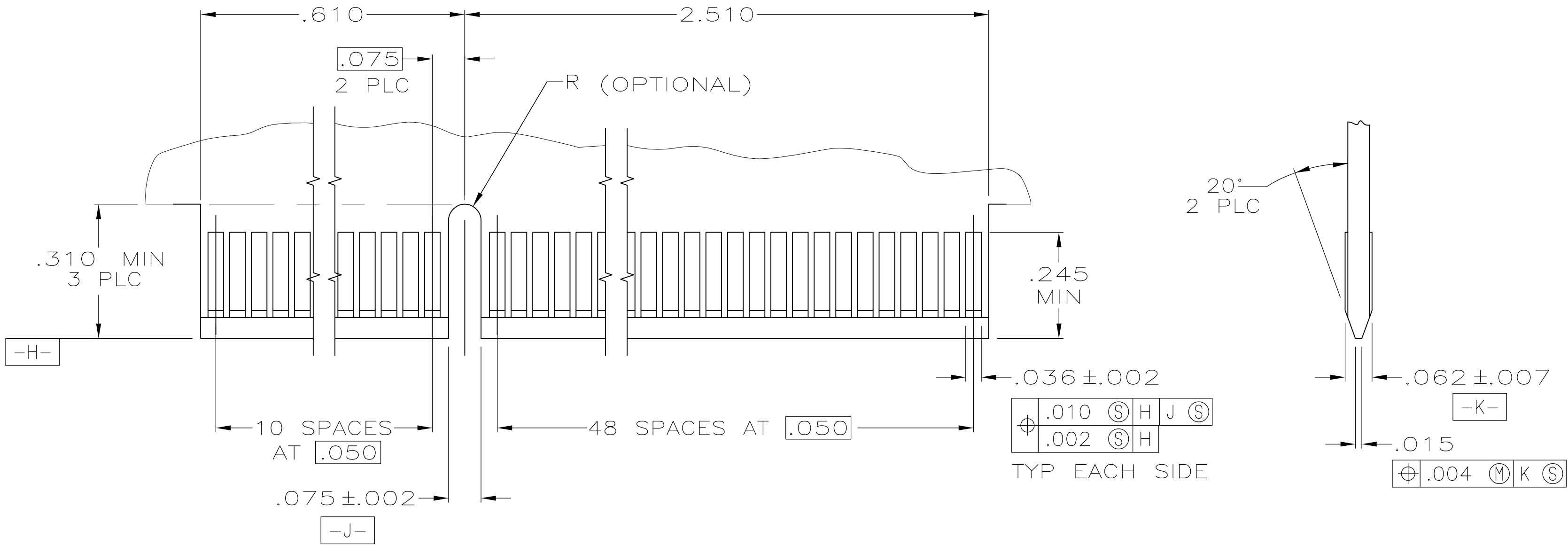
RECOMMENDED MATING BOARD EDGE CONFIGURATION
