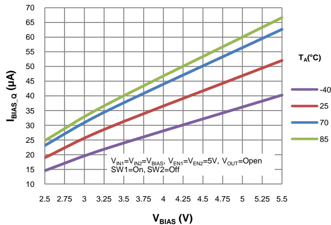
V_{BIAS} vs. QUIESCENT CURRENT (SINGLE CHANNEL)
