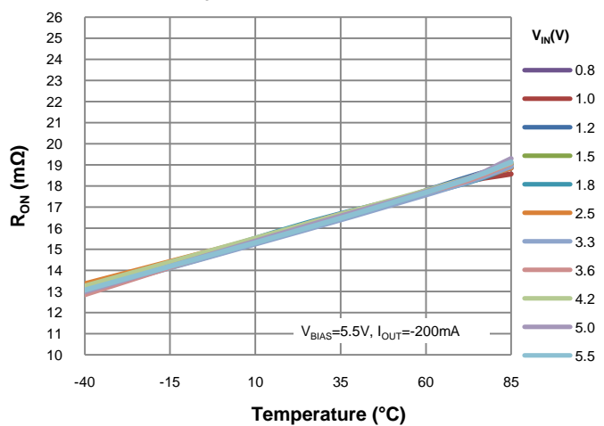
TEMPERATURE vs. R_{ON} ( V_{BIAS}=5.5\text{V} , SINGLE CHANNEL)
