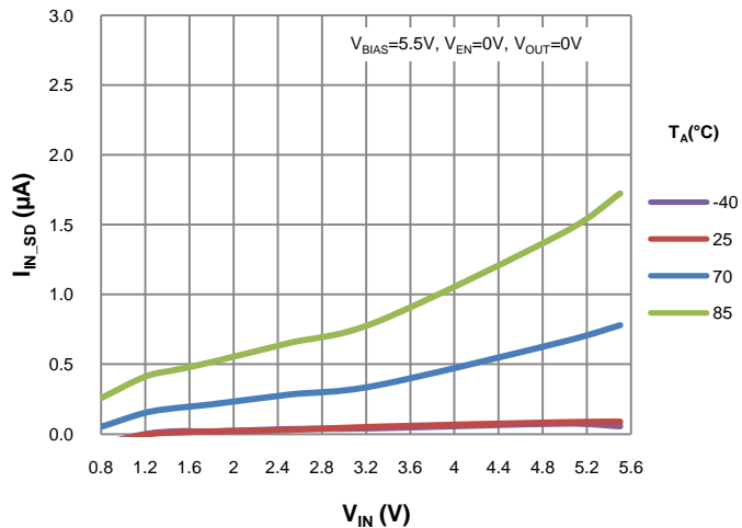
V_{IN} vs. OFF-STATE V_{IN} CURRENT (SINGLE CHANNEL)
