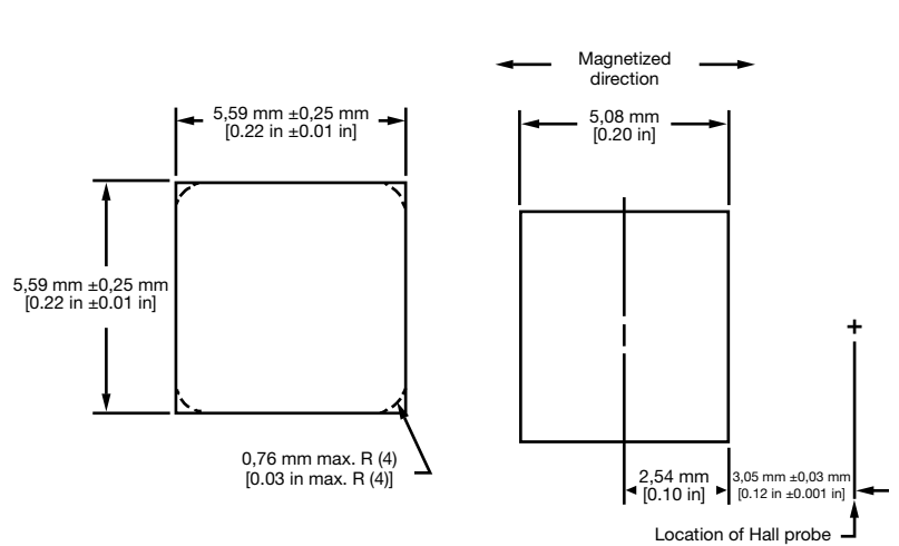
Figure 33. Rare Earth Pressed – 103MG8
