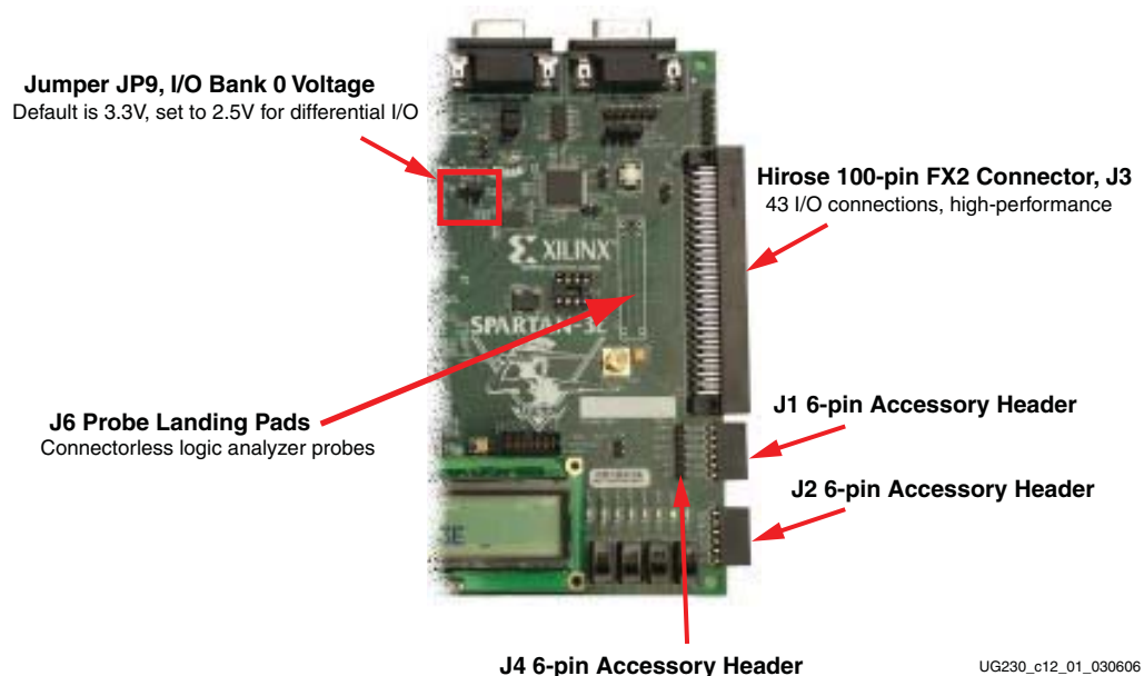
Figure 15-1: Expansion Headers
