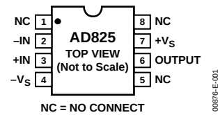
Figure 4. 8-Lead SOIC
